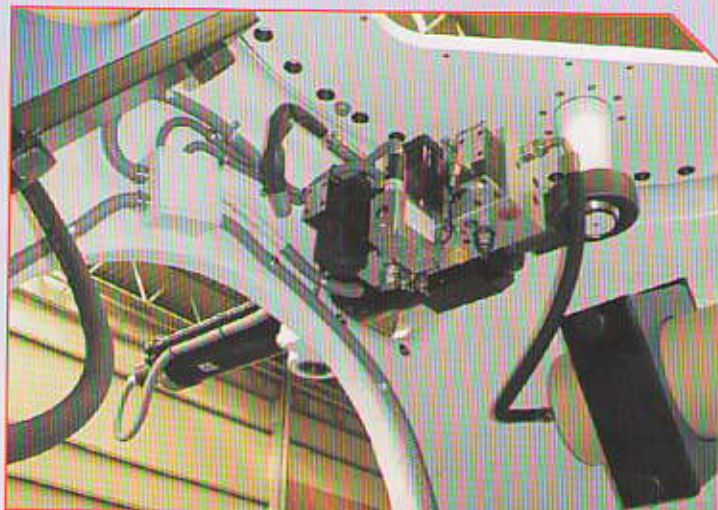
PITCH CONTROL AXIS WITH DDV ( DIRECT DRIVE VALVE)
