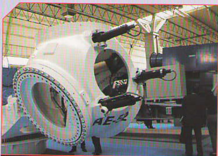
ROTOR OF THE WIND TURBINE WITH BLADE PITCH CONTROL AXIS
