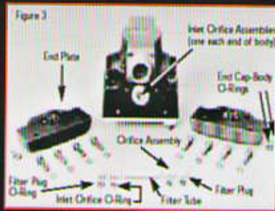
Moog 760 series
