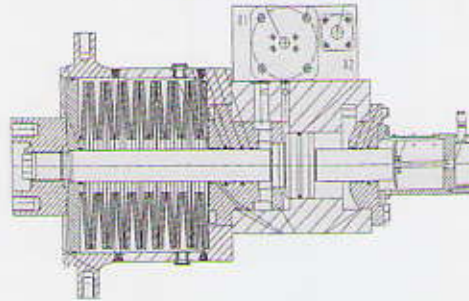
Disk Spring
