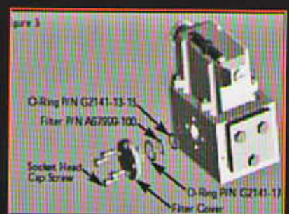
Moog 631 series
