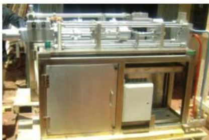
Main Rotor & Tail Rotor Actuator Test Rig
